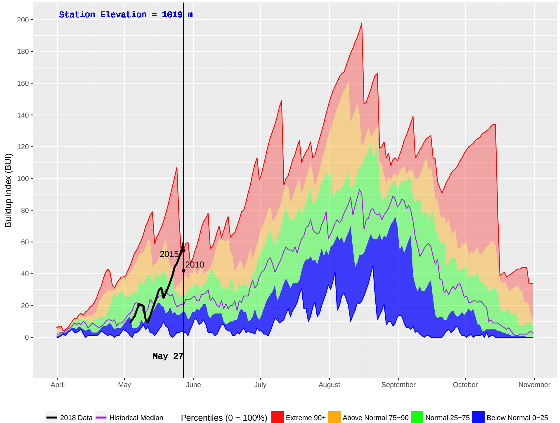
POWDER CREEK (380) : Historical (2001–2016) and Current (2018) Noon Buildup Index (BUI)
