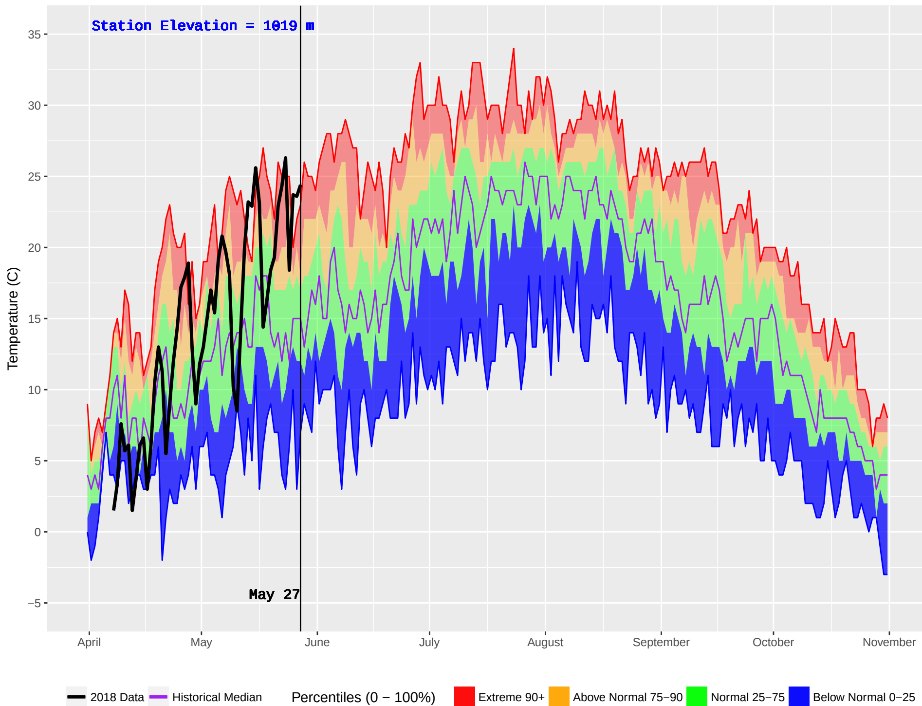
POWDER CREEK (380) : Historical (2001–2016) and Current (2018) Noon Temperature
