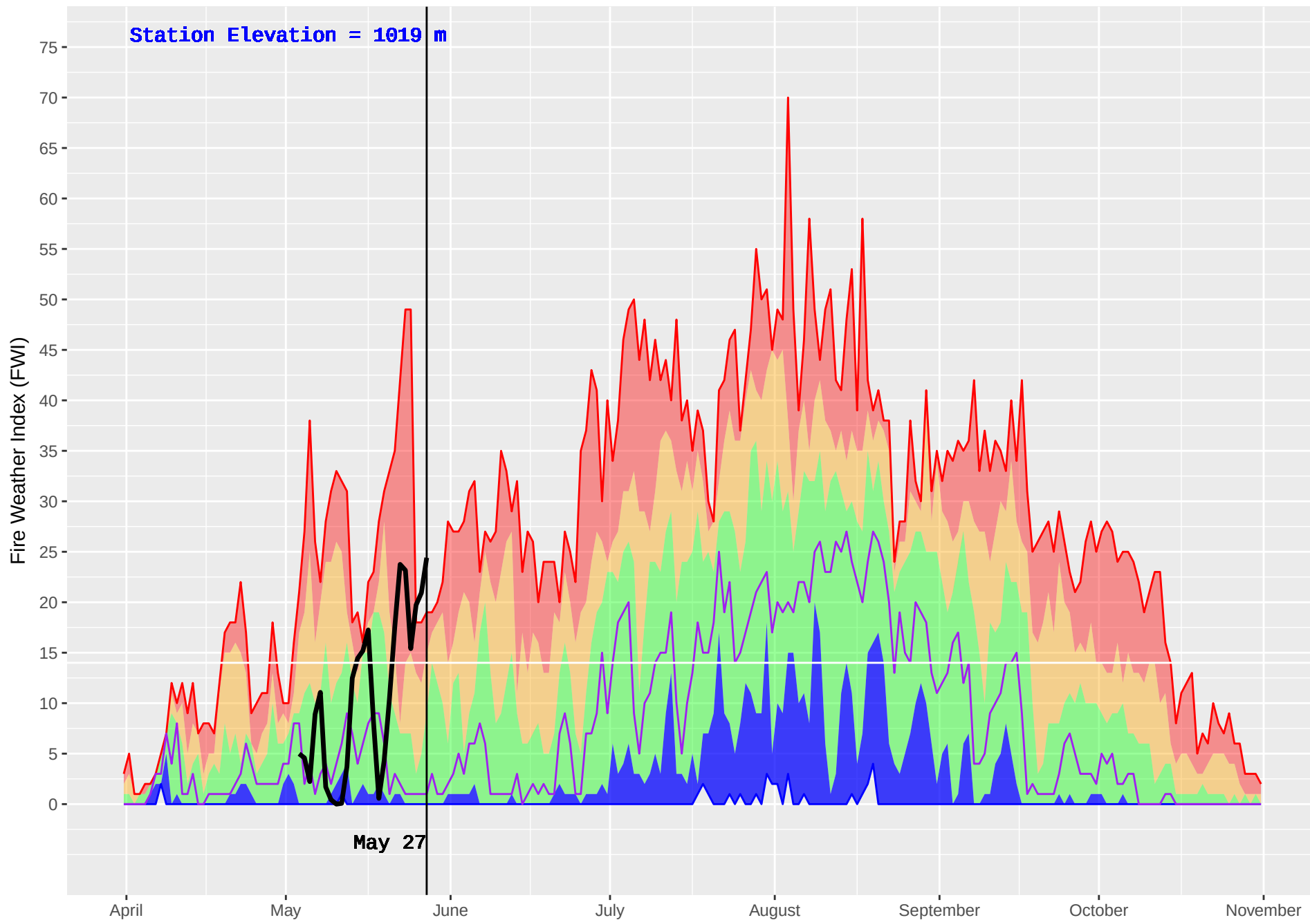
POWDER CREEK (380) : Historical (2001–2016) and Current (2018) Noon Fire Weather Index (FWI)
