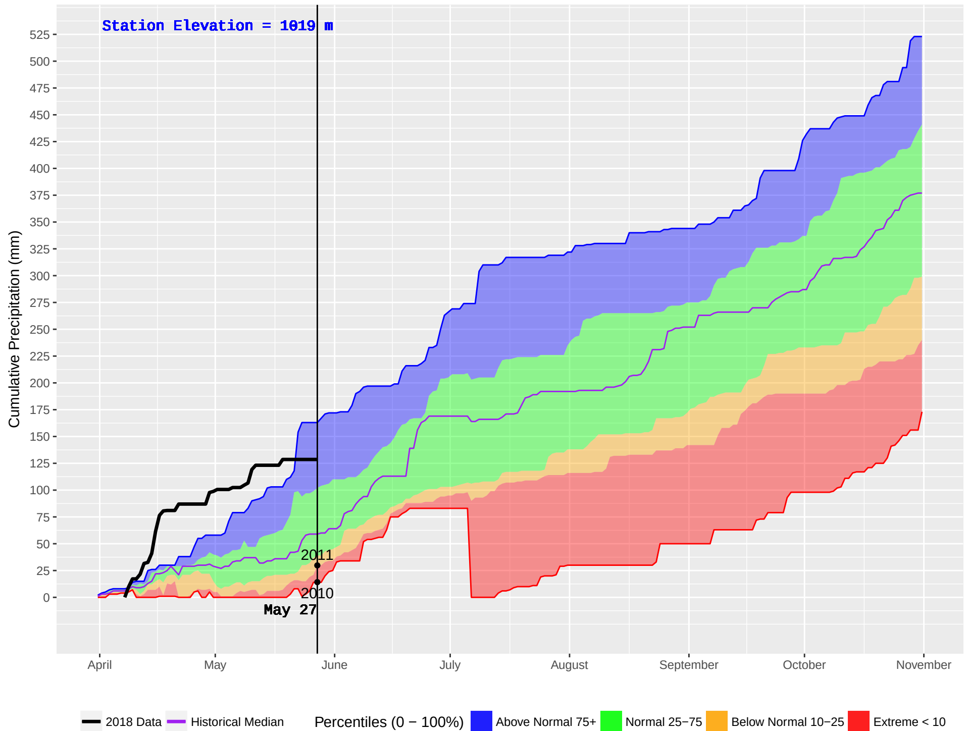
POWDER CREEK (380) : Historical (2001–2016) and Current (2018) Noon Cumulative Precipitation
